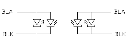
Backlight Circuit (No. of LEDs = 2*x2pcs) Scale=free
