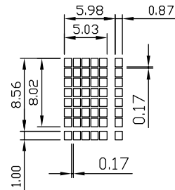
Pixels Details Scale=10/1
